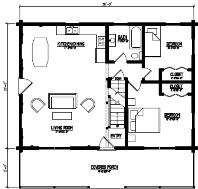
FIRST FLOOR PLAN 36' HIGH: 100 SQ. FT.
