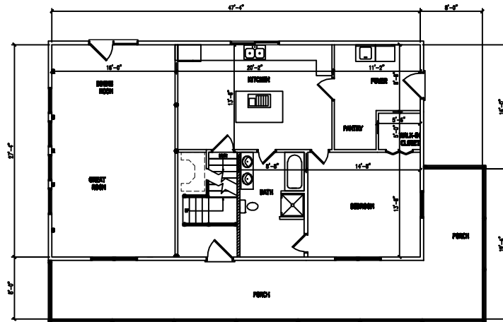
FLOOR PLAN
