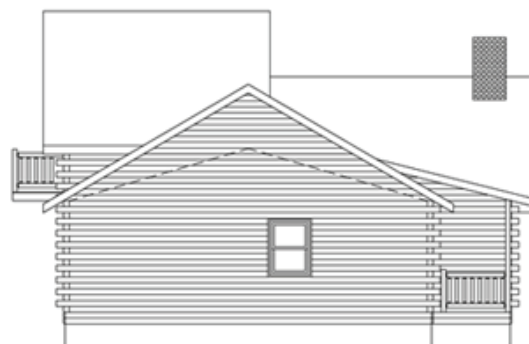
LEFT ELEVATION 3/16" = 1'-0"
